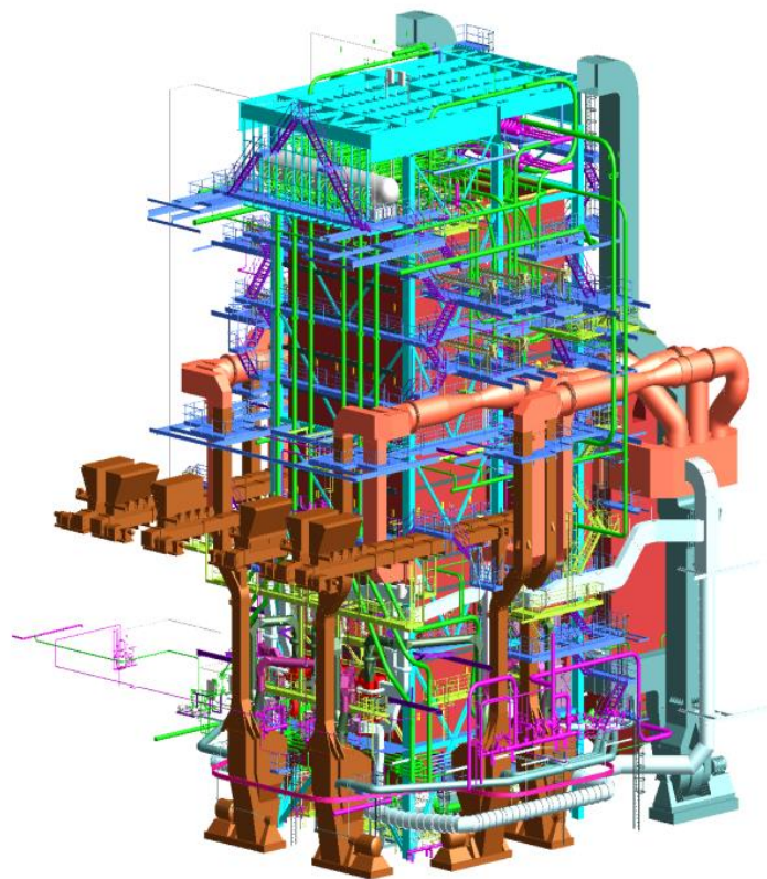
3D model of K6 boiler
